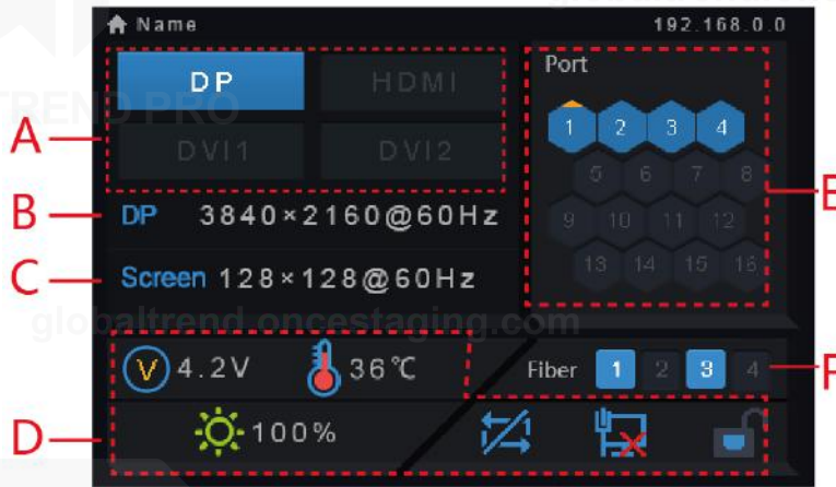
Figure 5-1 Home screen
